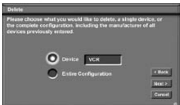
Figure 25. Delete screen
